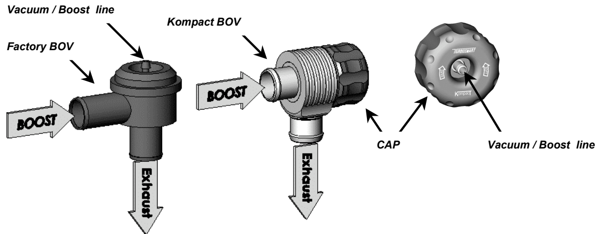
Figure 1 Orientation of Kompact PB BOV
